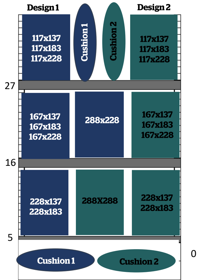
SPACE 1 SUNKEN BASE BAY LAYOUT
