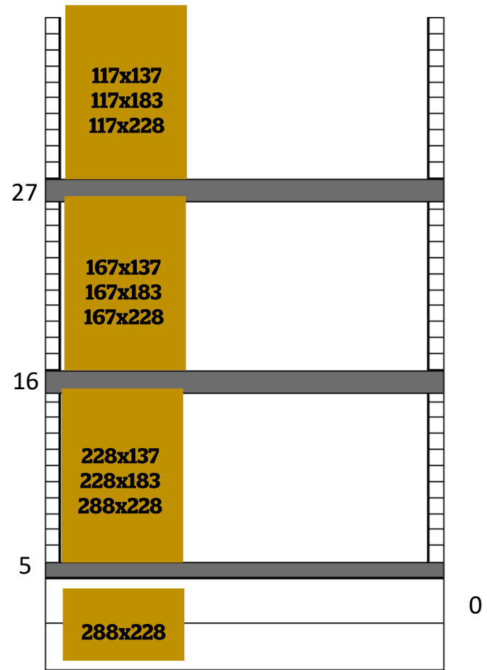
SPACE 0.33 NON CUSHION RANGE SUNKEN BASE LAYOUT
